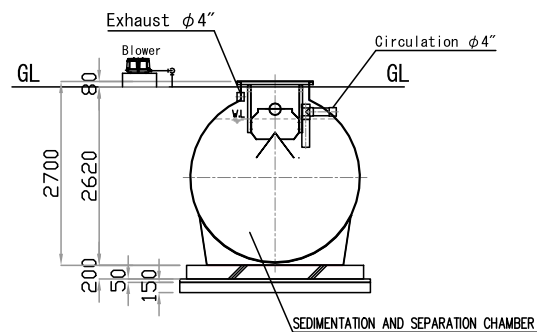
B-B SECTION
