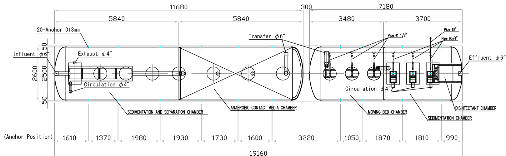
UPPER SECTION
