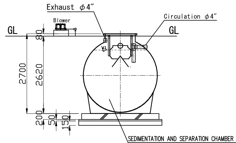
B-B SECTION
