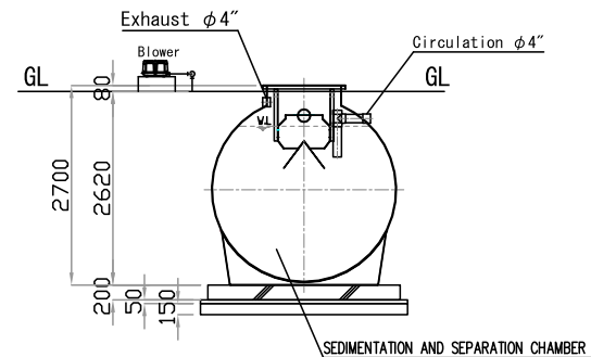
B-B SECTION
