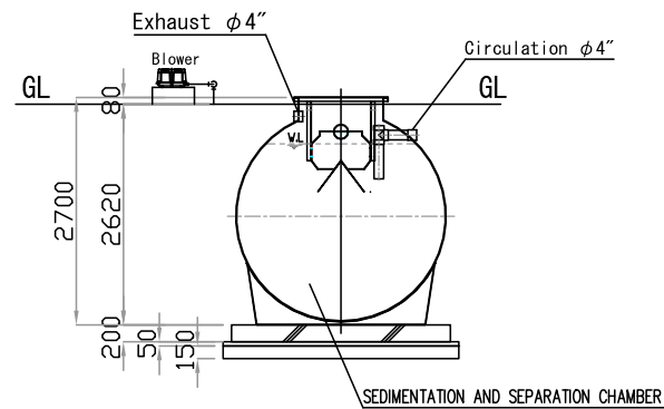
B-B SECTION
