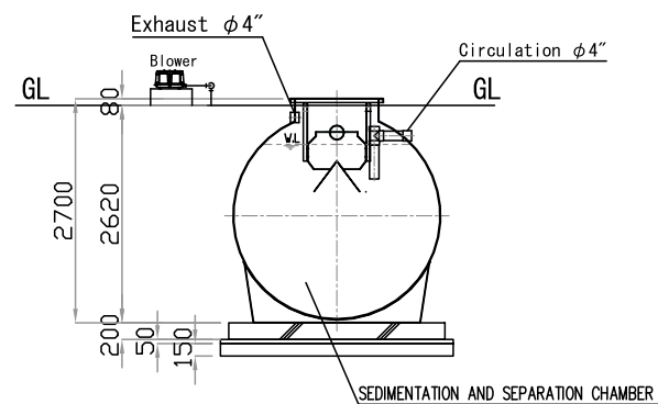
B-B SECTION
