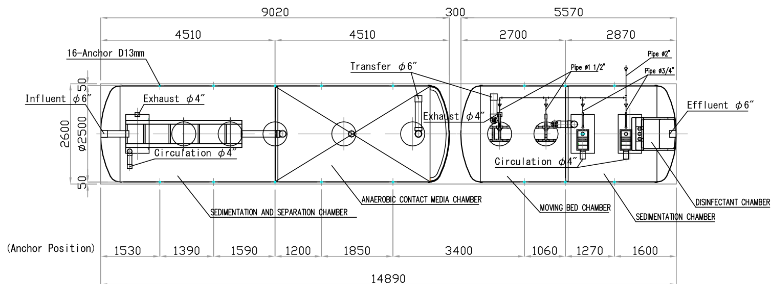
UPPER SECTION
