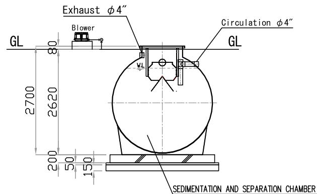
B-B SECTION
