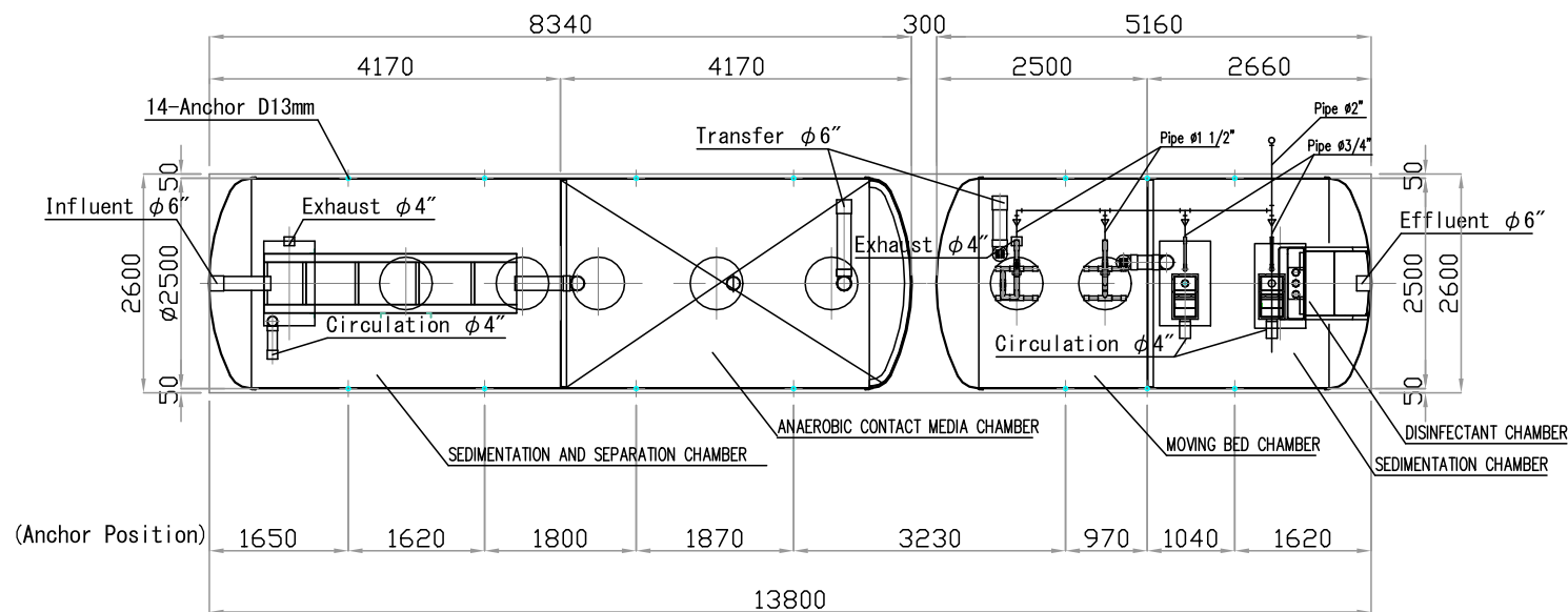
UPPER SECTION
