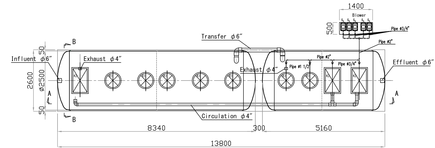
UPPER VIEW
