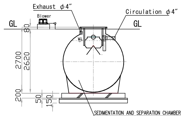
B-B SECTION
