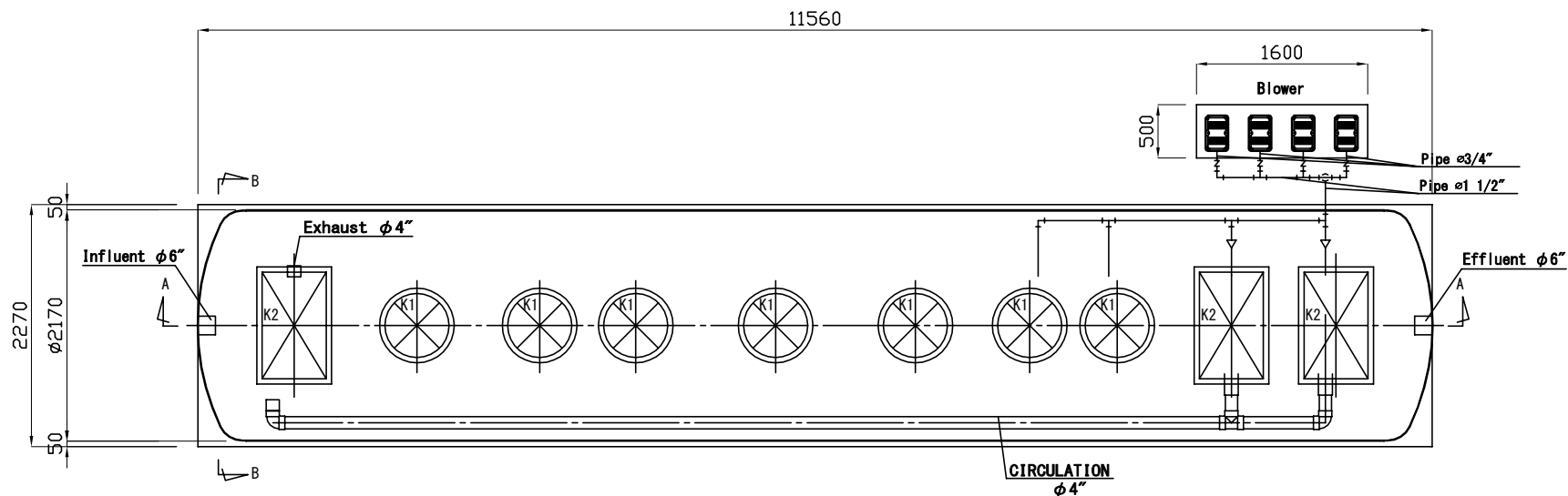
UPPER VIEW
