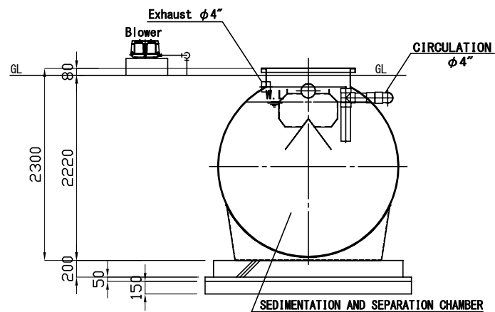
B-B SECTION
