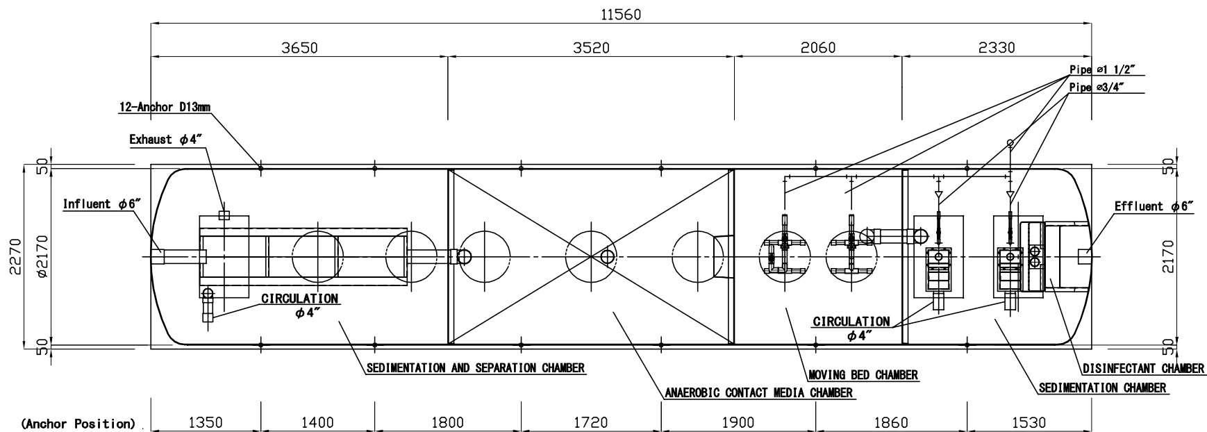
UPPER SECTION
