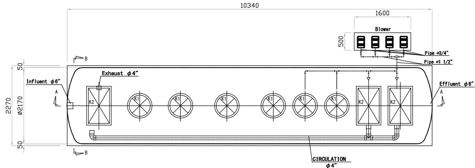
UPPER VIEW
