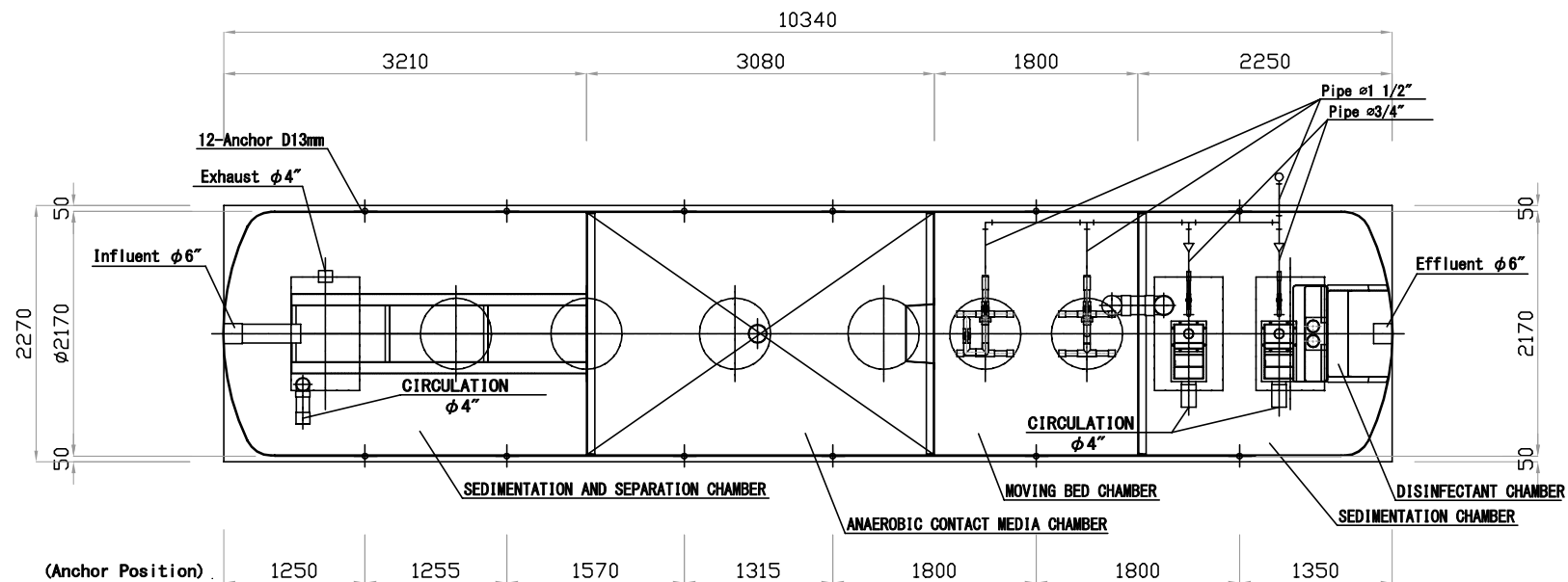
UPPER SECTION
