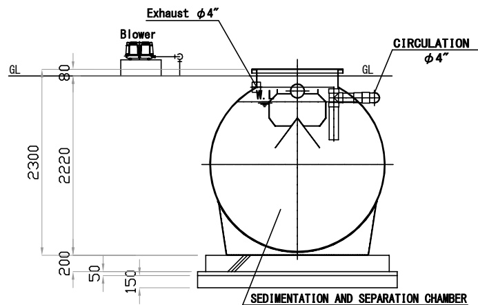
B-B SECTION
