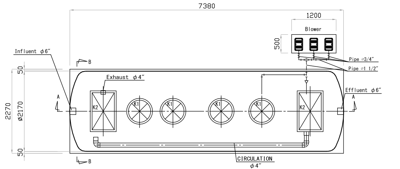
UPPER VIEW
