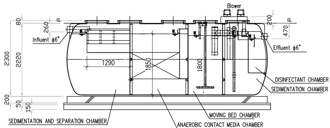
A – A SECTION
