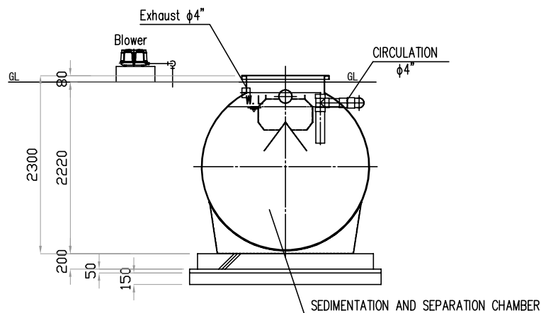
B – B SECTION
