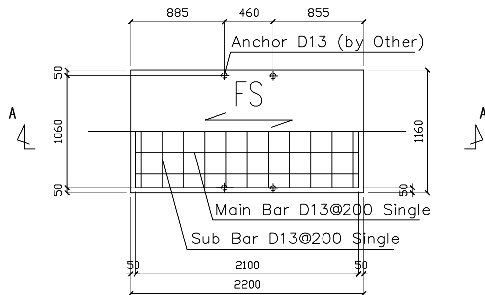
UPPER VIEW
