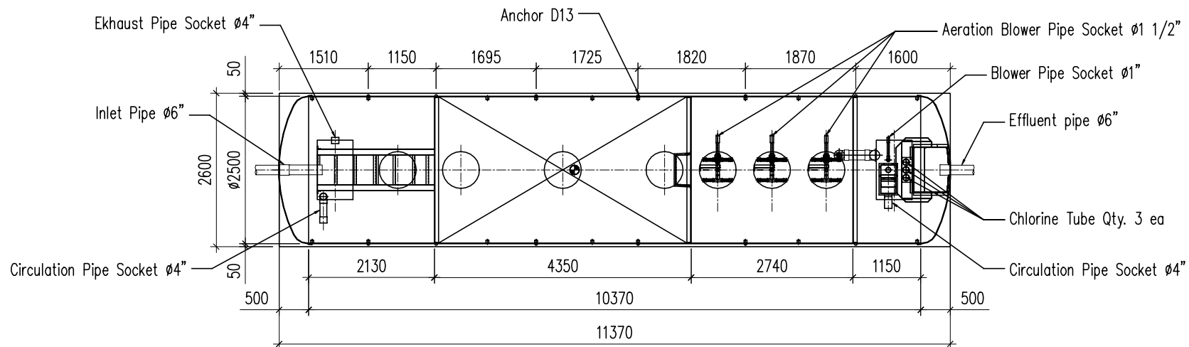
UPPER SECTION NTS
