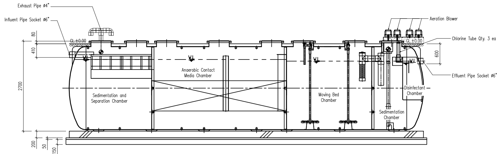
A - A SECTION NTS
