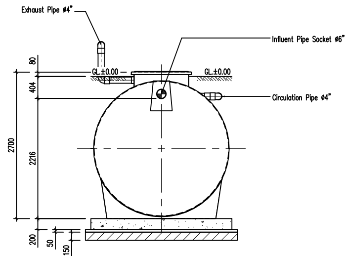
B - B SECTION NTS
