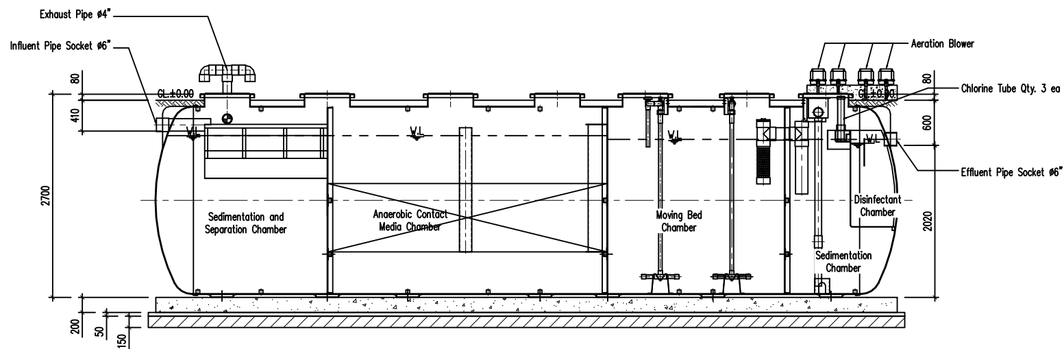
A - A SECTION NTS
