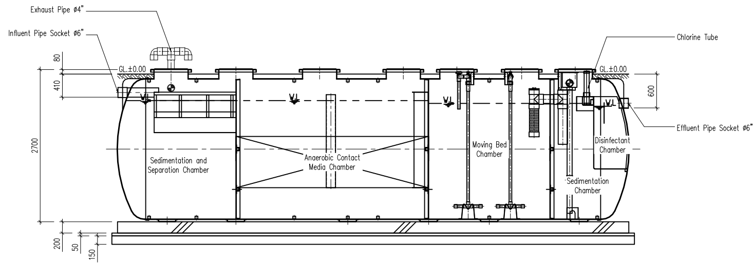
A - A SECTION NTS
