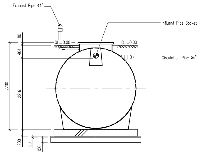
B - B SECTION NTS
