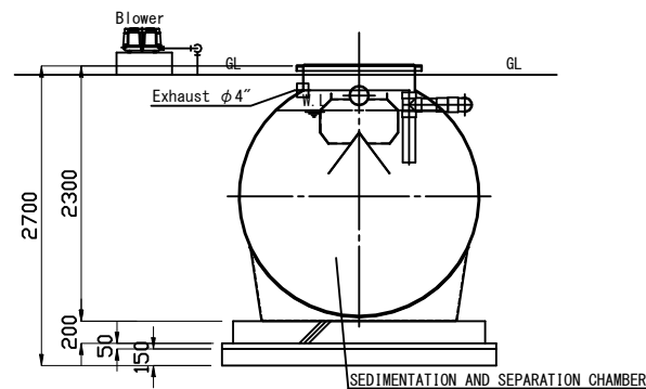
B-B SECTION
