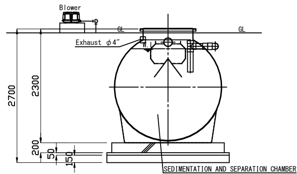
B-B SECTION
