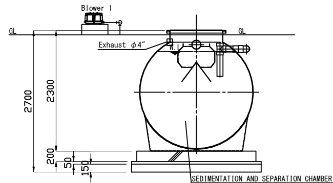
B-B SECTION
