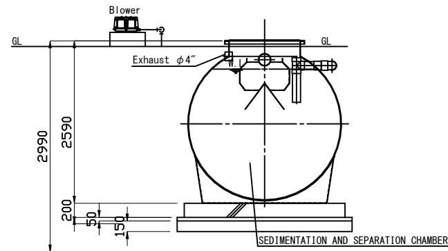
B-B SECTION
