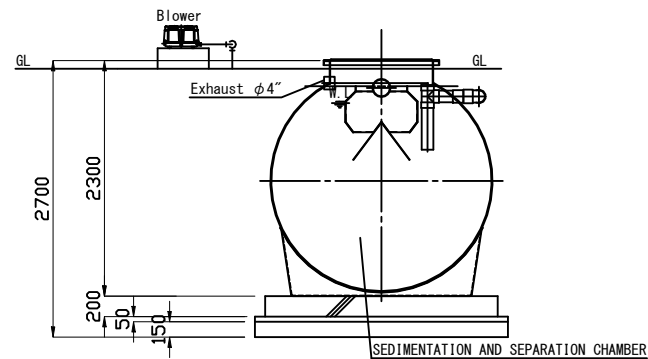
B-B SECTION
