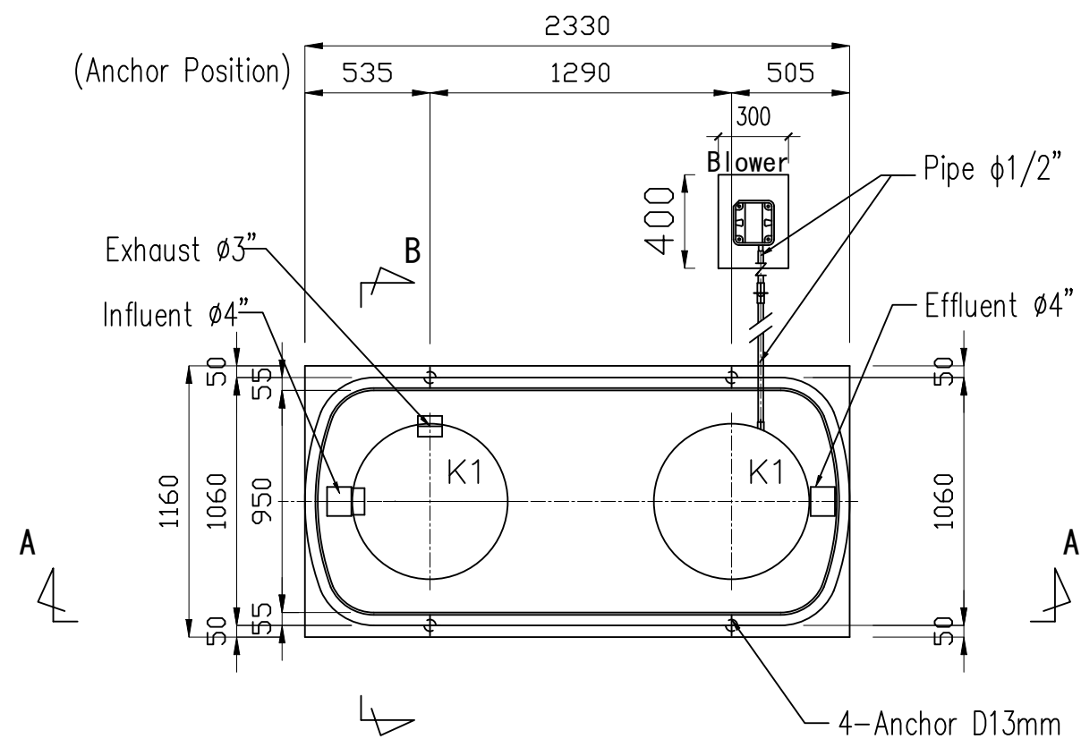
UPPER VIEW
