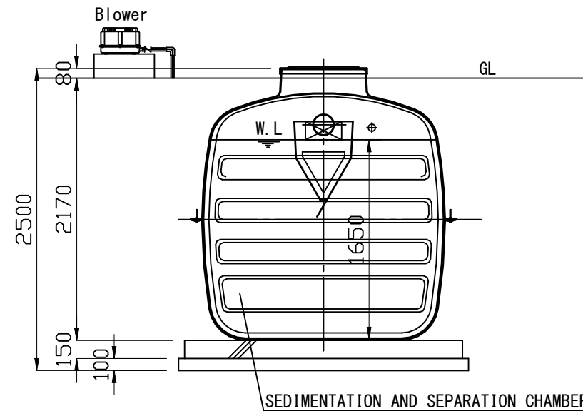
B-B SECTION
