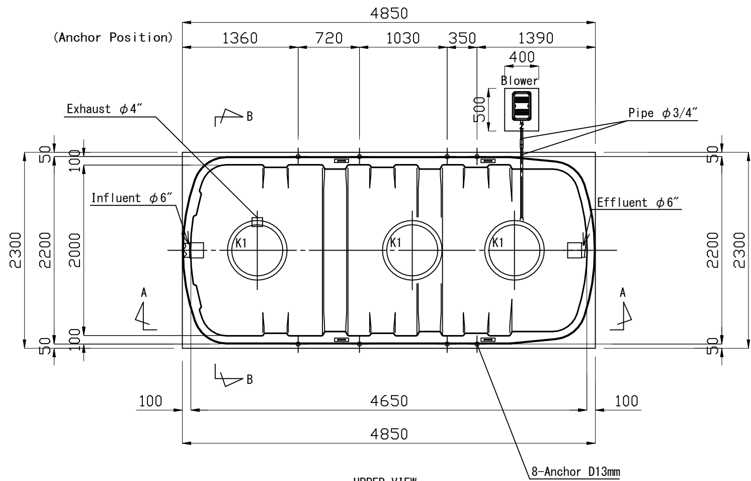
UPPER VIEW
